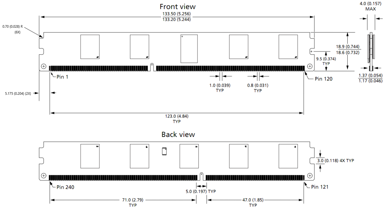
Figure 1 - Package Dimensions_ HXMSH4GP03A2F1VL16K
